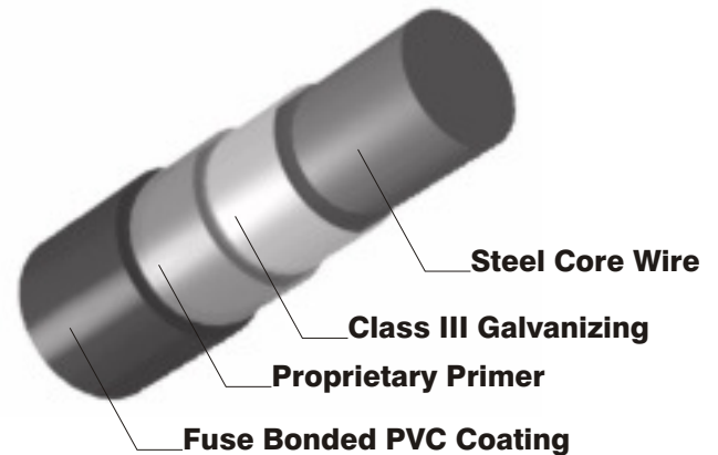
Cross Section Shepherd PVC Coated Wire
